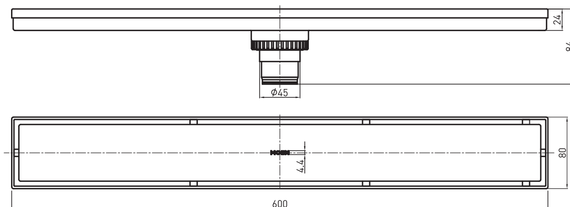
LONG FLOOR DRAIN(ST.ST) MODELS:207322
