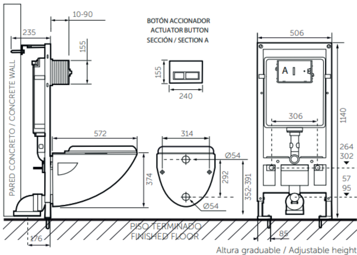
VISTA LATERAL / LATERAL VIEW
